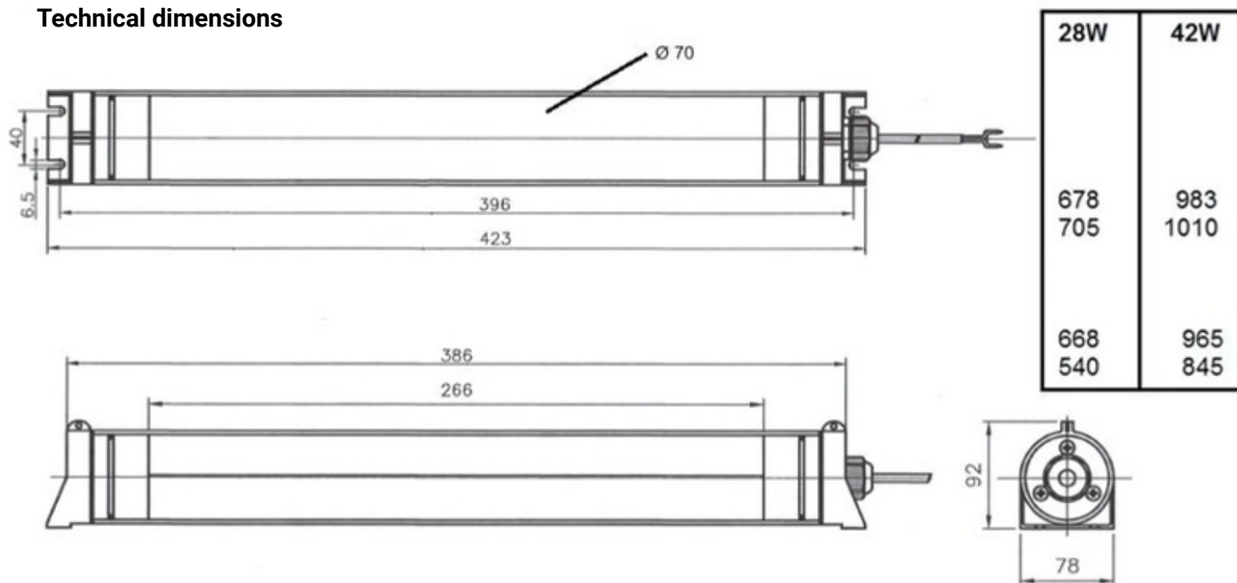
Technical dimensions
